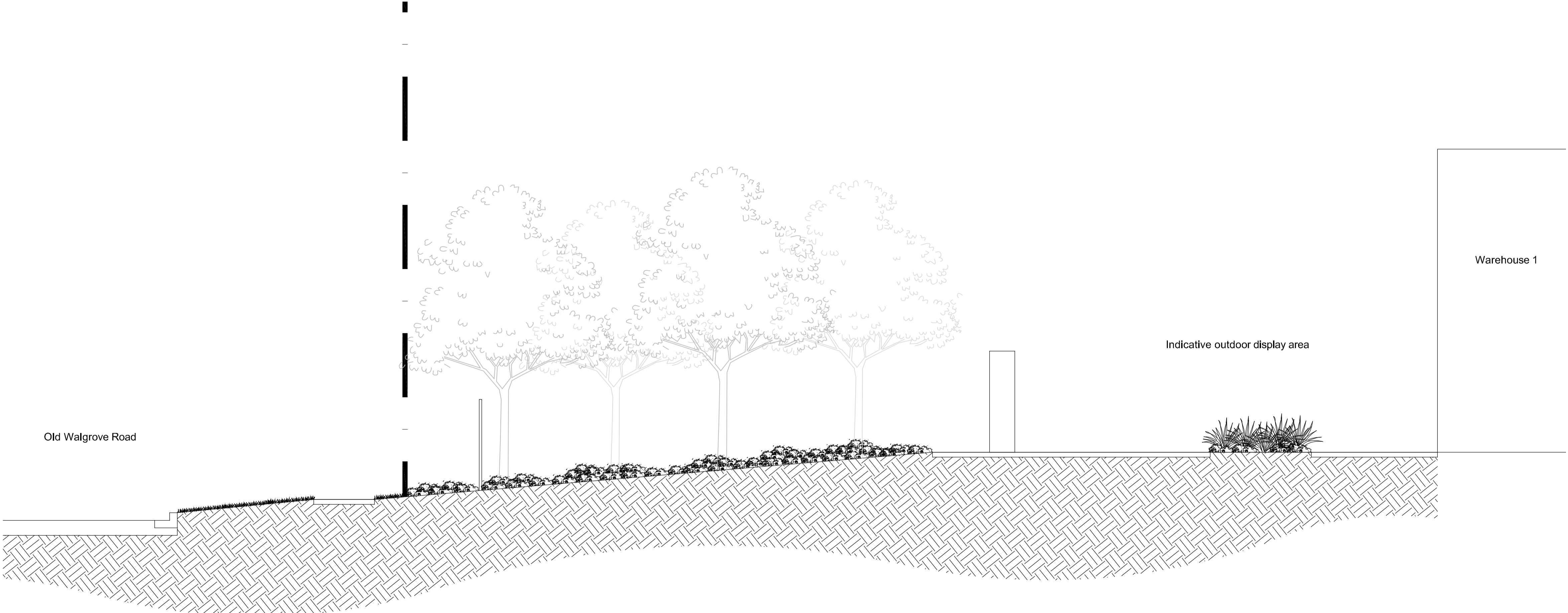
02 Landscape Section 601 1:50
