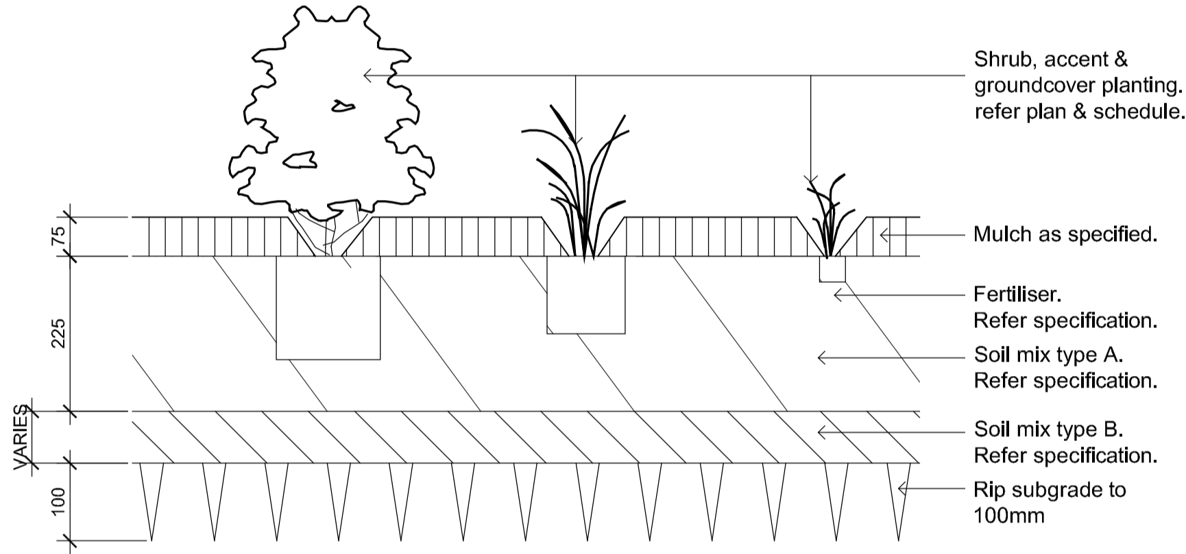
03 Shrub, Accent & Groundcover Planting on Grade 501 1:10
