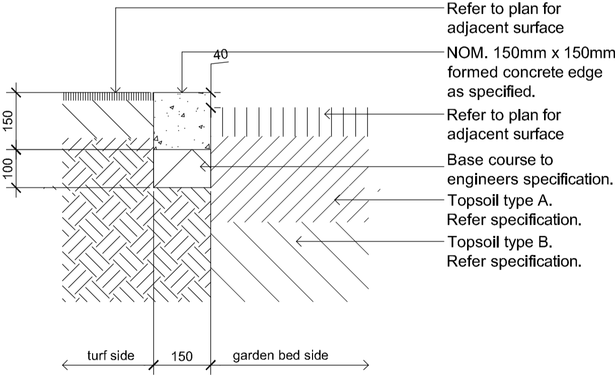
04 Typical Concrete Edge 501 1:10
