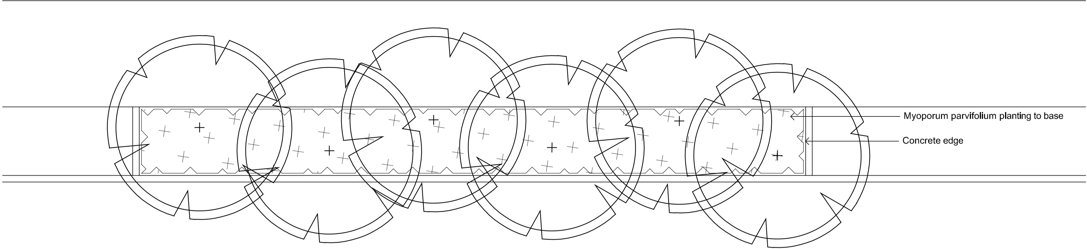
01 Street Tree Planting Detail 501 1:50
