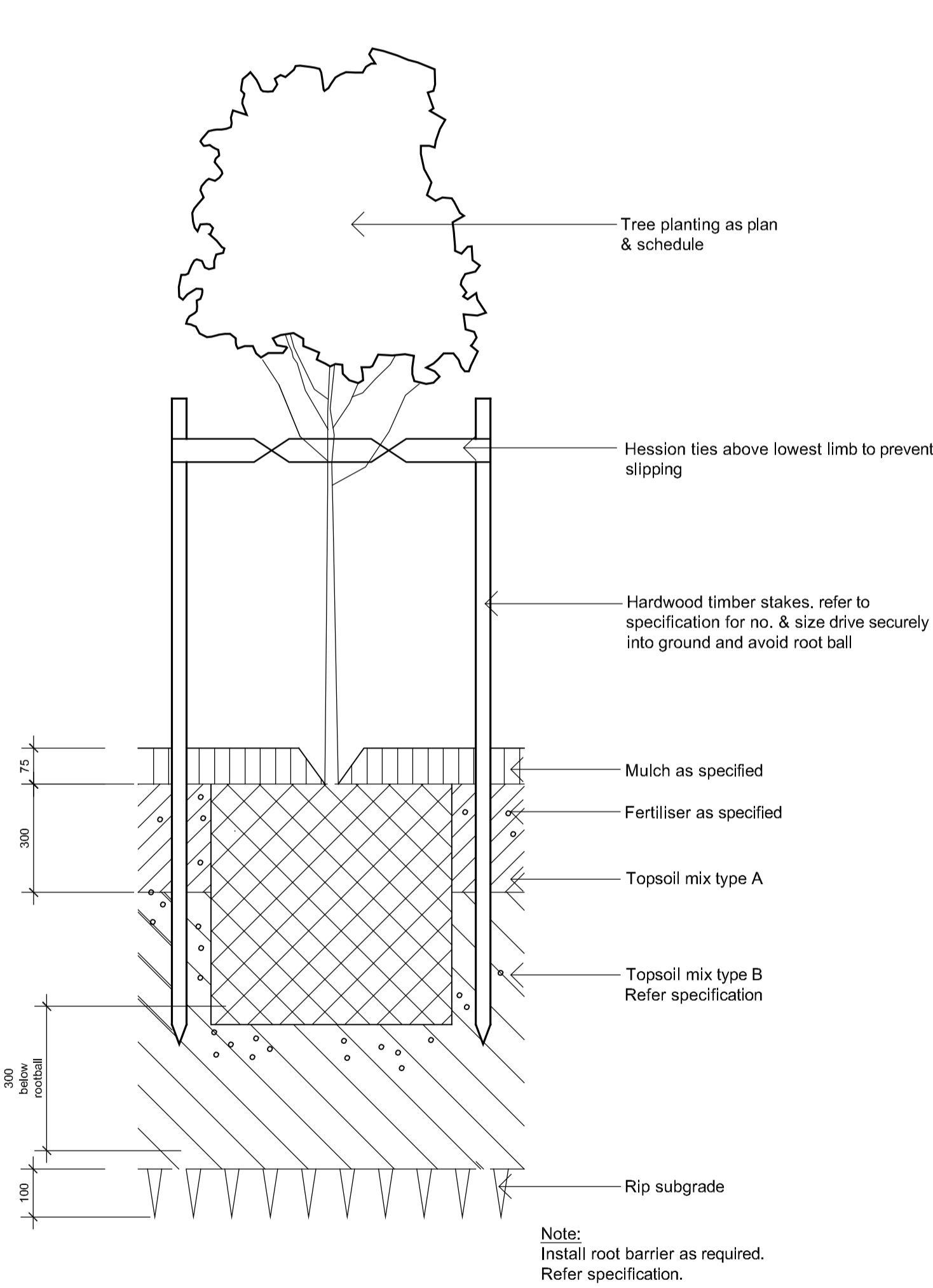
02 Detail - 75-200L Tree Planting on Grade 501 1:10
