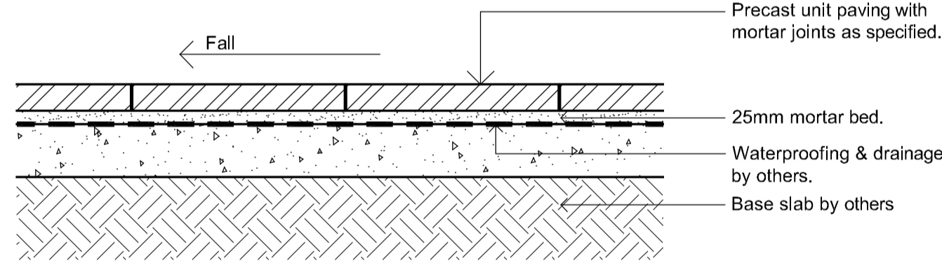
06 Precast Unit Pavers on Suspended Slab 501 1:10
